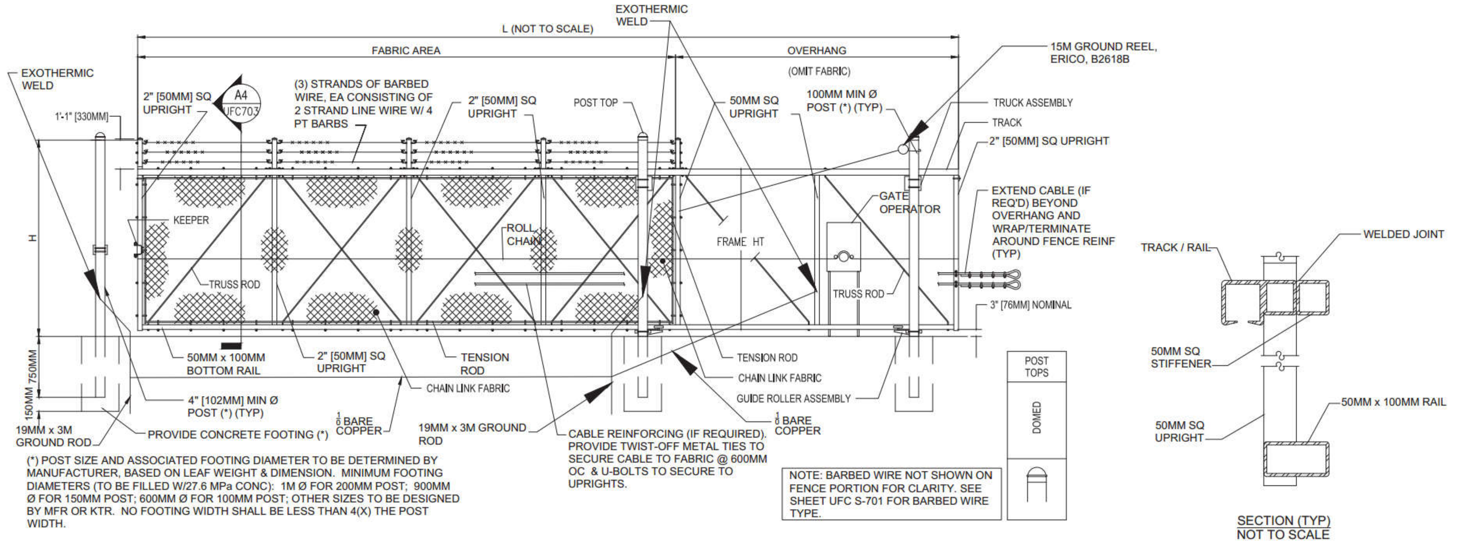
A1 TYPICAL SINGLE CANTILEVERED SLIDING GATE ELEVATION - (4) BAYS SHOWN SCALE N.T.S.
